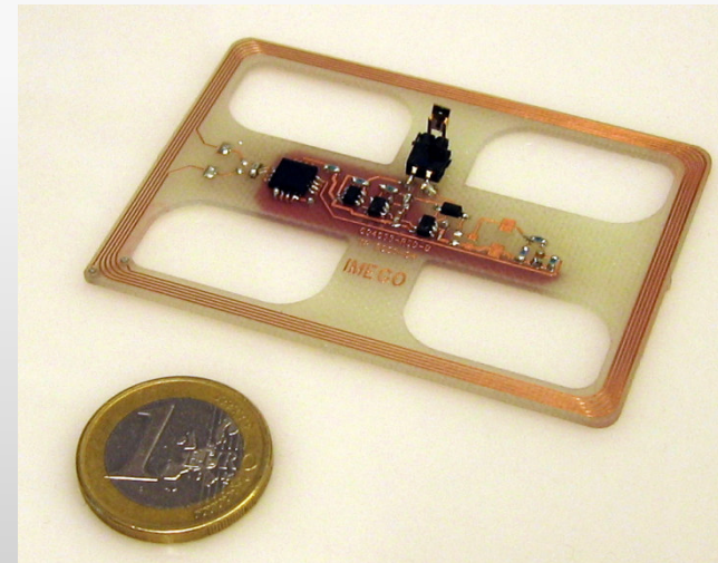
RFID tag IDS-SL13A with internal temperature sensor together with Imego's humidity sensor and interface electronics
