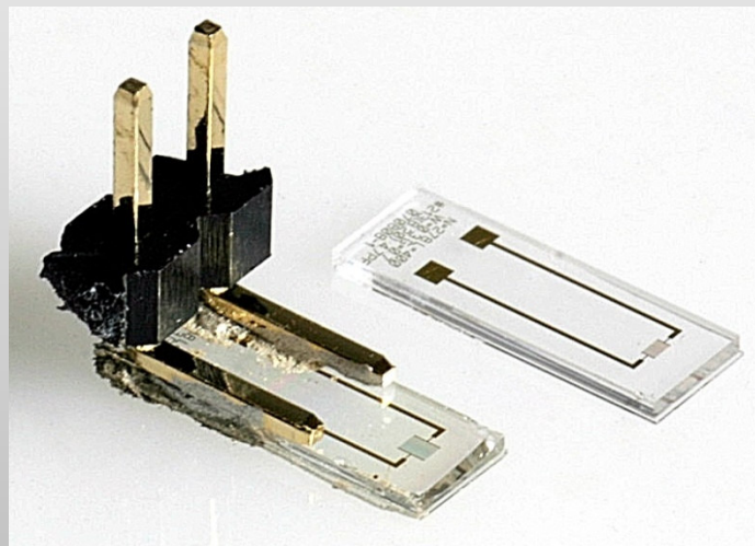
Imego's capacitive humidity sensor
