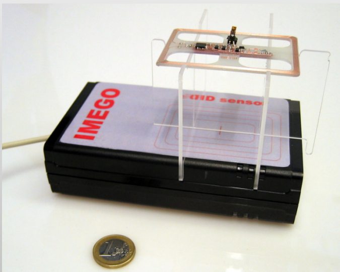
RFID reader IDS-R13MP (inside box) and RFID sensor tag
